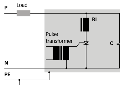
Saturating chokes in series with thyristors
