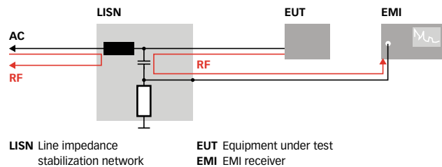
Measurement principle for line-conducted voltage measurements
