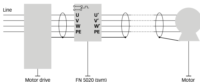
Drive with symmetrical sinusoidal filter
