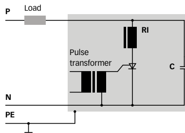
Saturating chokes in series with thyristors
