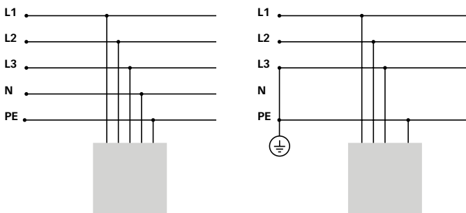
TN-S distribution networks
