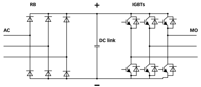
RB Rectifier bridge IGBTs Insulated gate bipolar transistors MO Motor output
