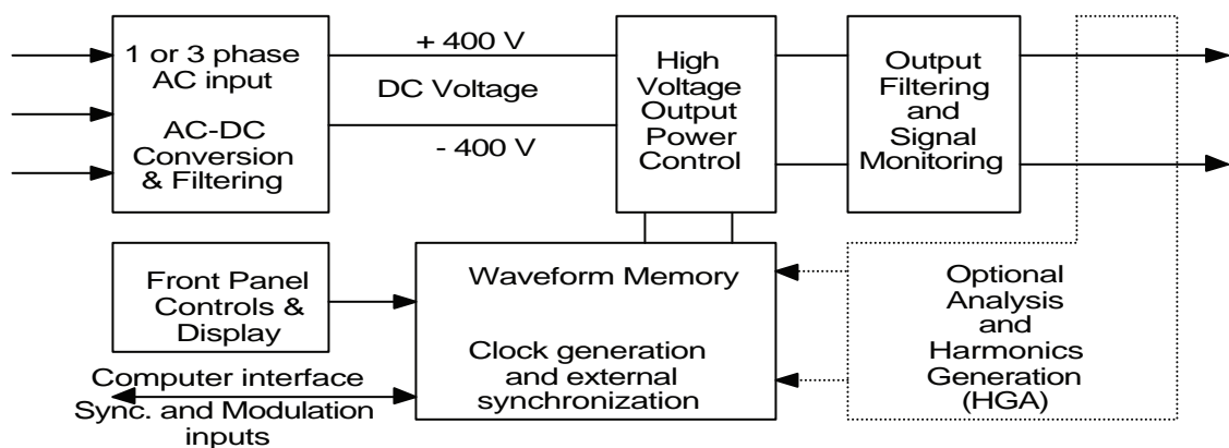
Figure 5 : Power Source Block Diagram
