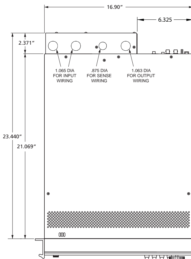
Top View
