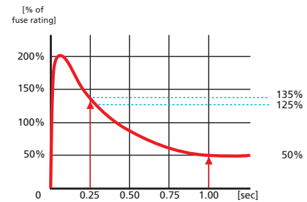
Fast output current profile created through sequence programming supporting fuse rating test
