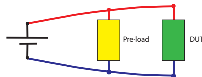
The pre-load should draw a current at least up to 75% of the DUT, to significantly improve the output voltage over- & undershoots
