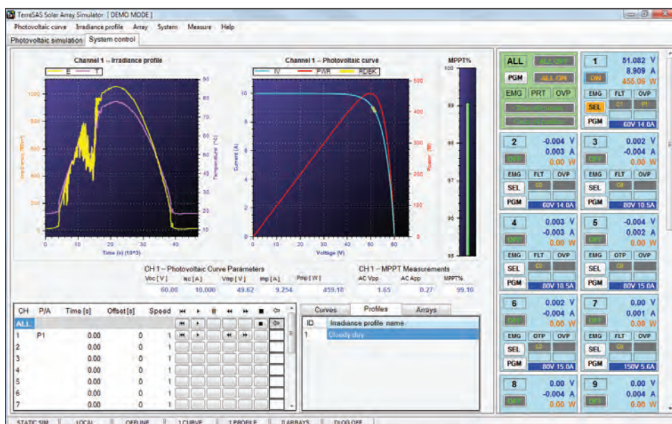
Figure 3. The TerraSAS real-time display updates 20 times per second, allowing you to see how well the simulator tracks the simulated solar panel's I-V curve.
