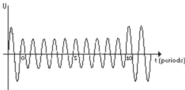
Fig. 3: Typical Voltage dips test.
