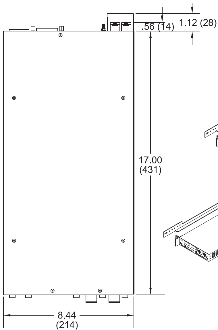
Top View
