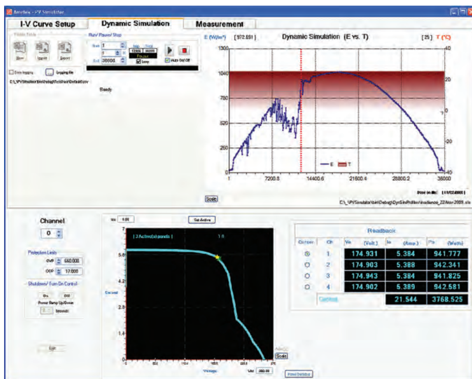
Dynamic simulation showing changes in Irradiance and Temperature over time
