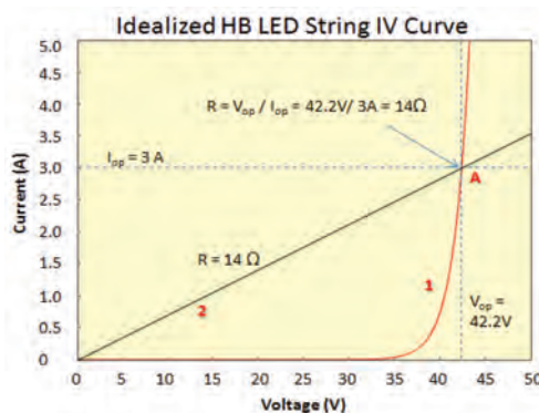
Fig. 2 Typical IV Chart
