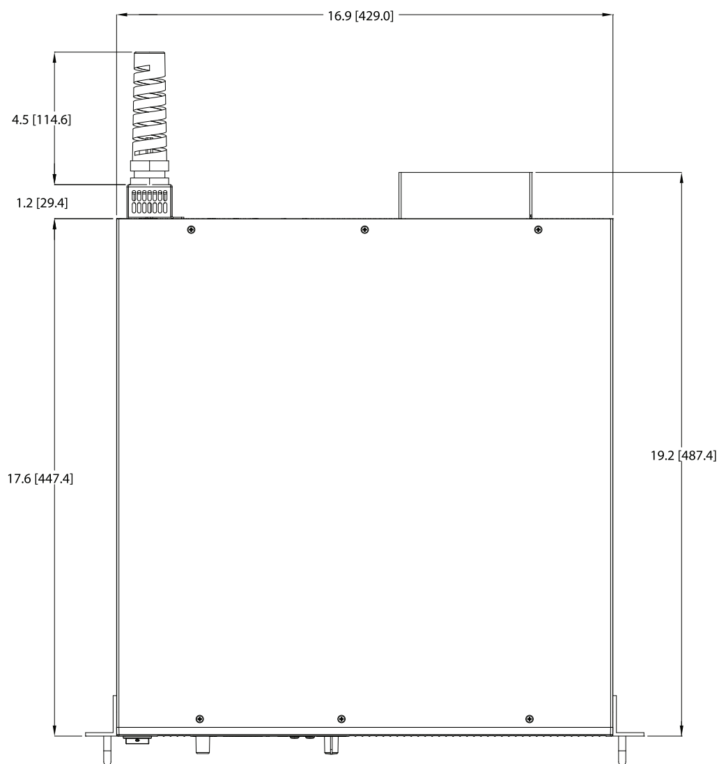
TOP VIEW
