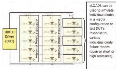
Fig. 4 Simplified Matrix Configuration
