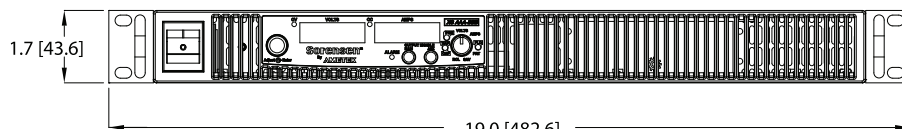
FRONT VIEW
