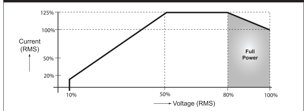
Constant Power AC Mode - Available Max. AC Current
