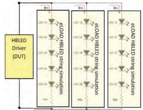
Fig. 5 Parallel String Configuration
