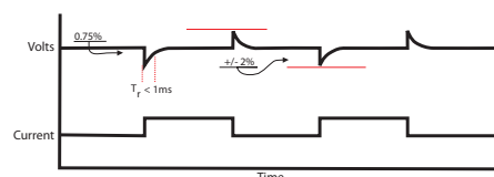
Typical transient response specification for a switch-mode programmable DC power supply: At a current change of 50% of maximum output current range, the DC output voltage will over- or undershoot not more than 2% of its set voltage. And recover within 0.75% of the set voltage, within less than 1ms.
