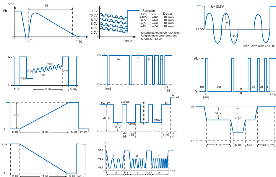
Figure 2. Examples of power simulation test scenarios
