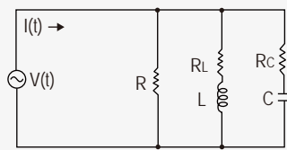
Parallel rlc
