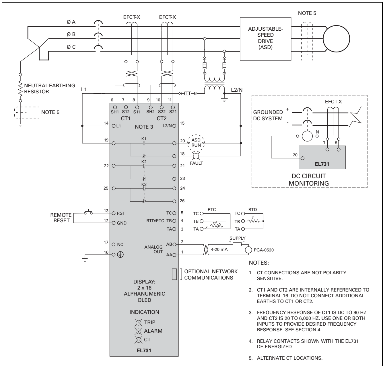
FIGURE 4. Connection Diagram.
