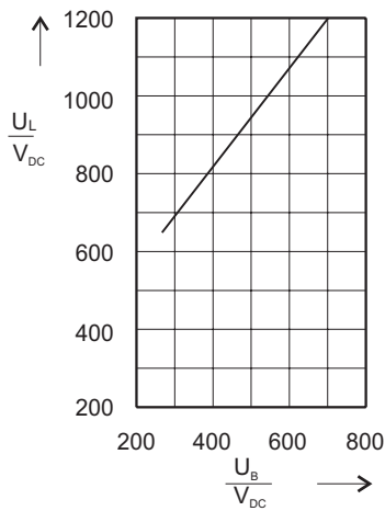
Arc Voltage-Diagram
